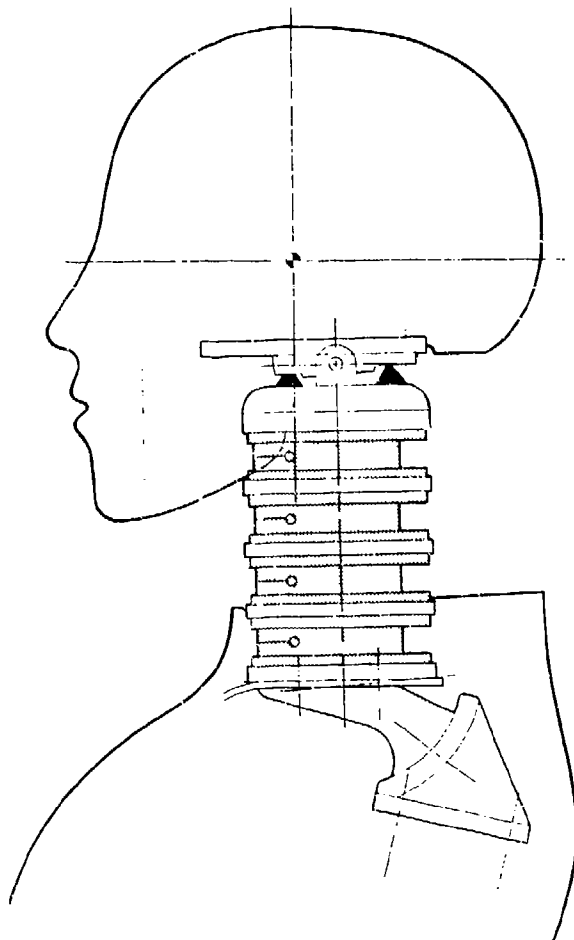
FIGURE 48. HYBRID III NECK.
