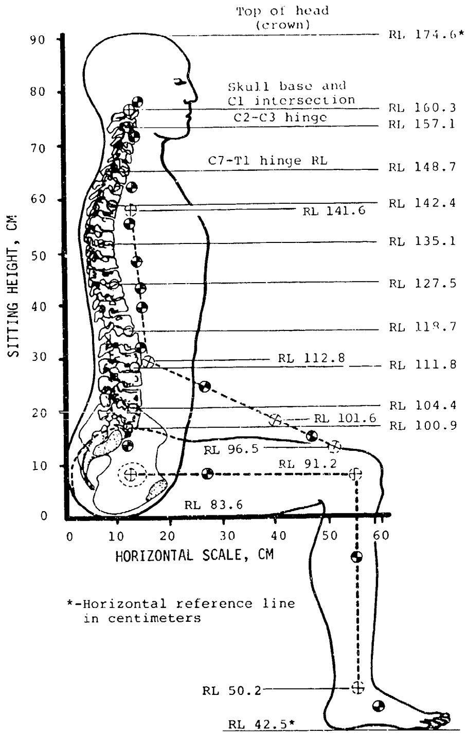
FIGURE 43. SITTING SKELETAL JOINT LOCATIONS BASED ON A 50TH-PERC NTILE MALE ARMY AVIATOR. (FROM REFERENCE 81)
