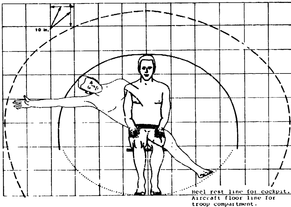
FIGURE 38. LAP-BELT-ONLY EXTREMITY STRIKE ENVELOPE - FRONT VIEW.
