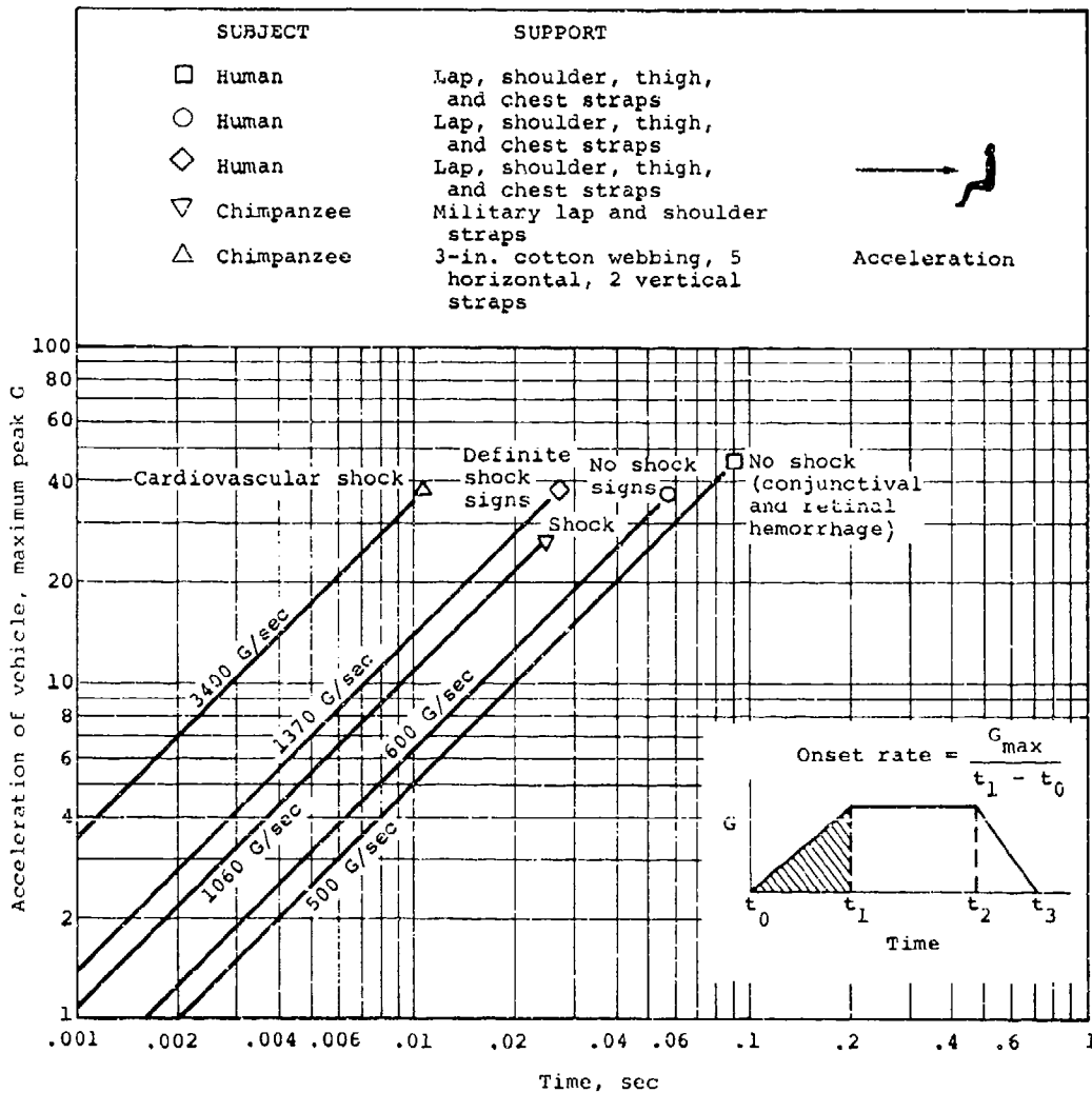
FIGURE 10. INITIAL RATE OF CHANGE OF SPINWARD ACCELERATION ENDURED BY VARIOUS SUBJECTS. (FROM REFERENCE 13)
